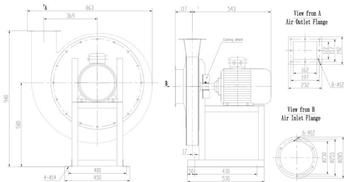
(GA -DRAWING)
