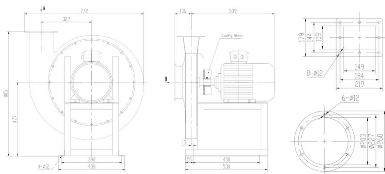
(GA -DRAWING)
