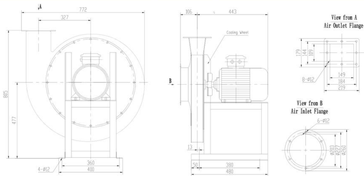
(GA -DRAWING)
