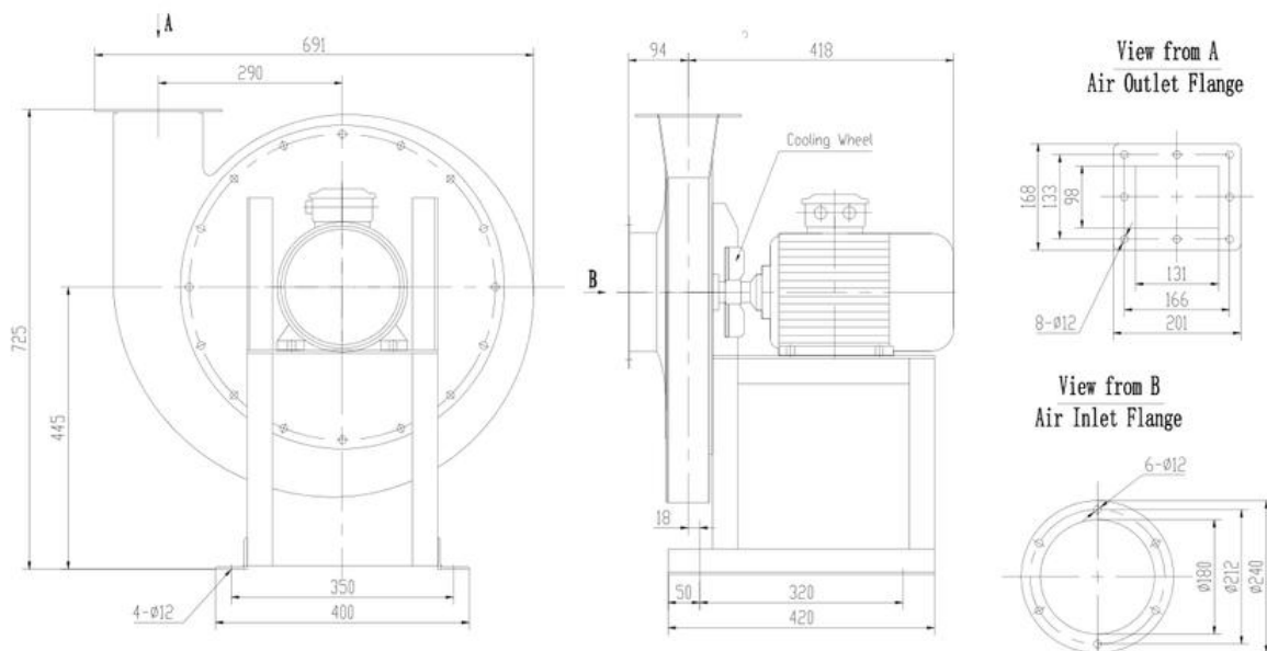
(GA -DRAWING)
