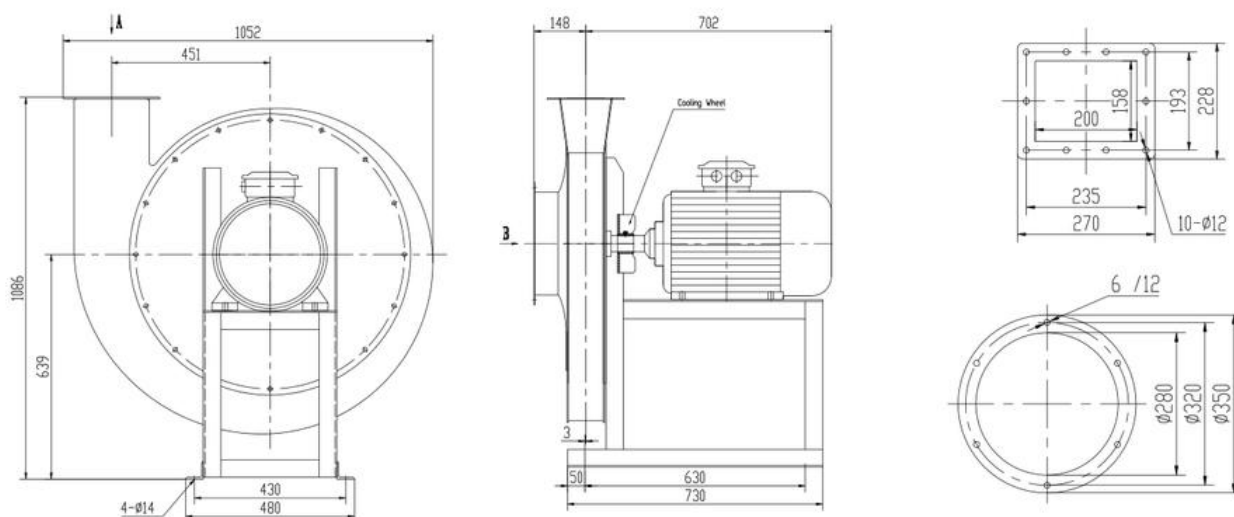
(GA -DRAWING)
