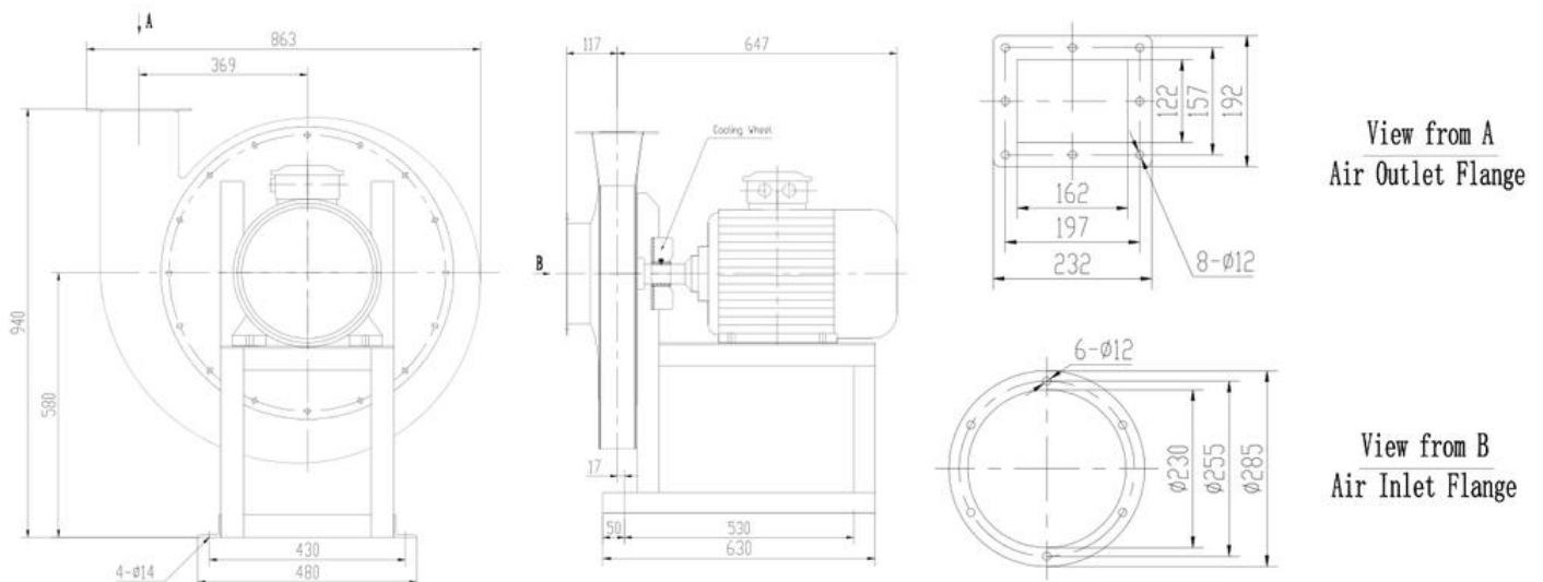
(GA -DRAWING)
