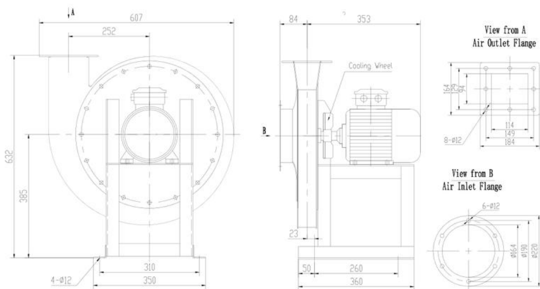
(GA -DRAWING)
